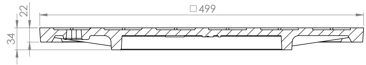
SECTION A-A SCALE 1 : 3.5
