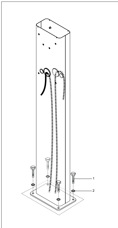
Fig. 03: Final mounting
